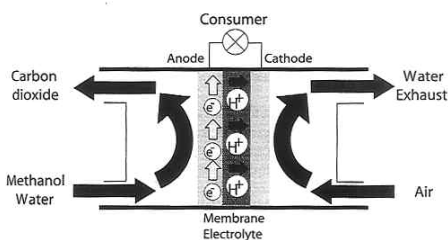
Diagram of a Direct Methanol Fuel Cell
